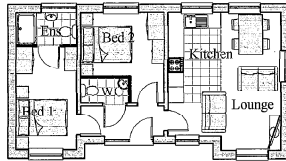
Plot 7 FLOOR PLAN Office Conversion 0 1 2 3 4 5m 1:100
